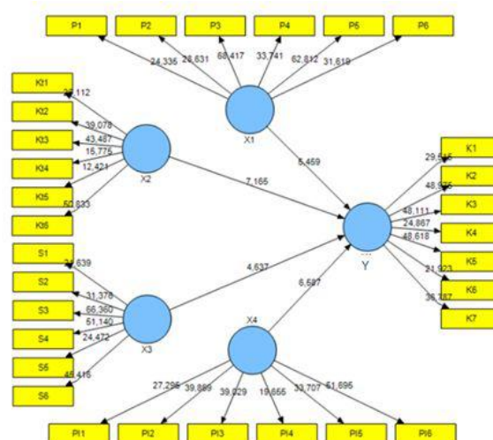
Figure no. 1 structural model with t-value.
